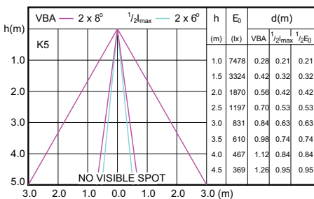
LED Lamps, MAS LEDspotLV D 11-50W AR111 G53 830 8D
