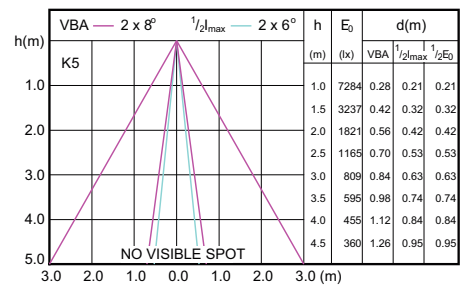
LED Lamps, MAS LEDspotLV D 11-50W AR111 G53 827 8D
