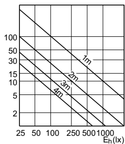
SDAC_LEDspotL_0144-Accent diagram
