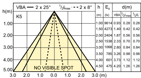
SDBE_LEDspotL_0144-Beam diagram
