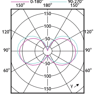
— 0-180° — 90-270°
